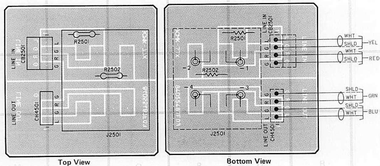
● Phono Plate P.C. Board
