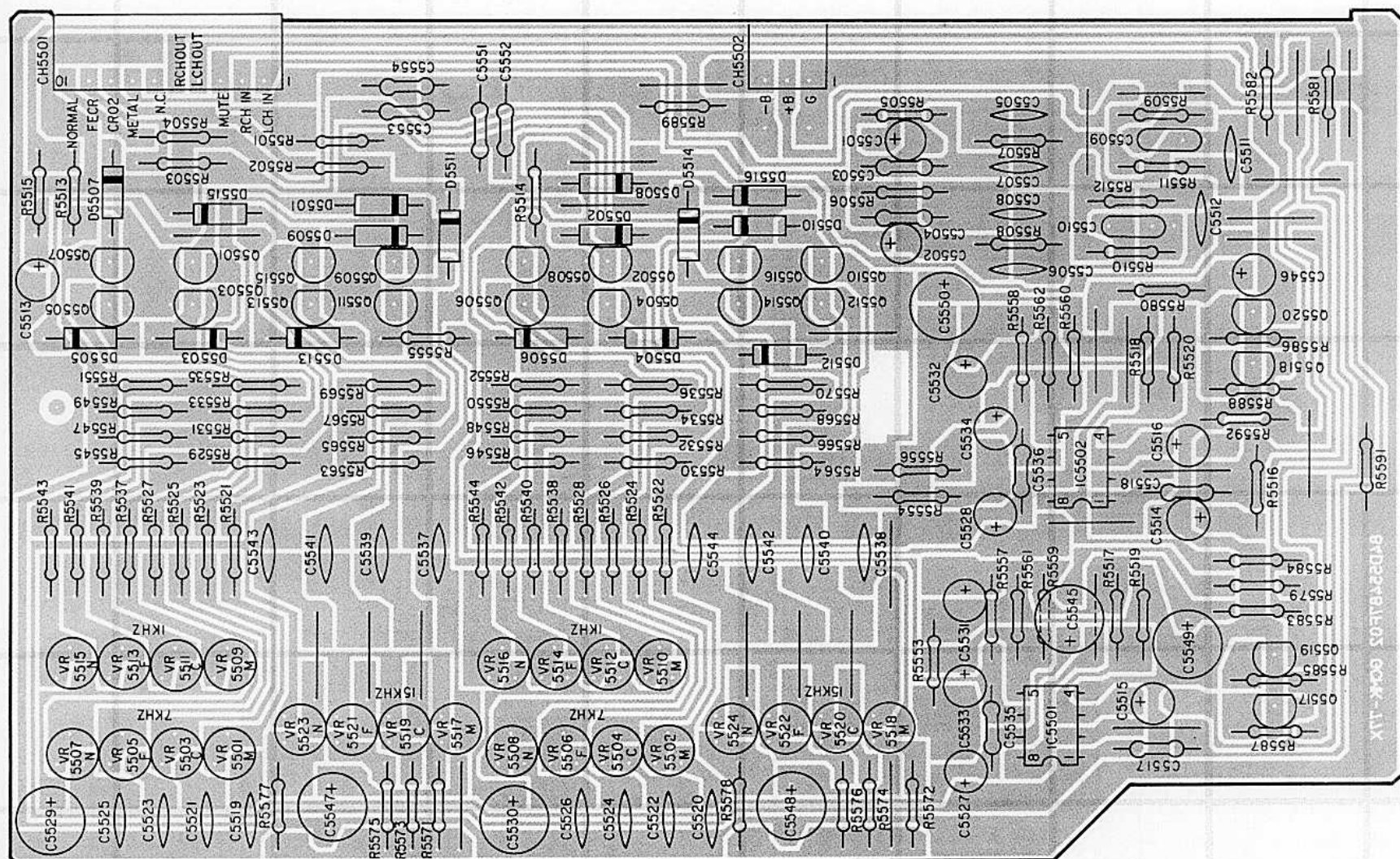
Top View
