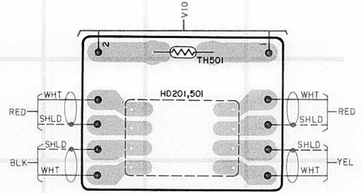
Bottom View
