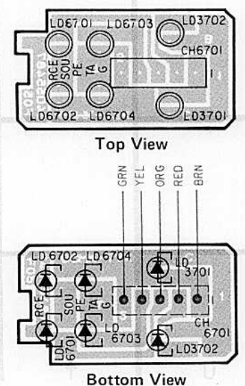
● LED P.C. Board
