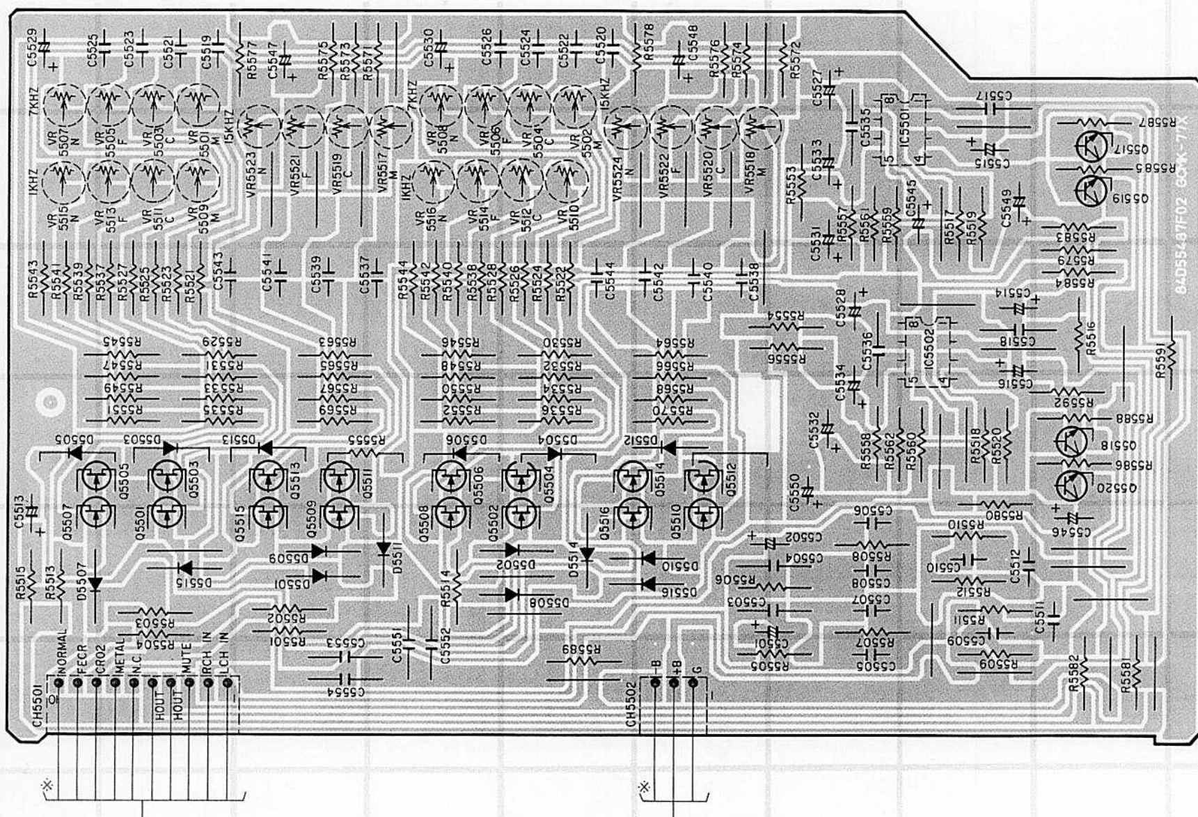
Bottom View
